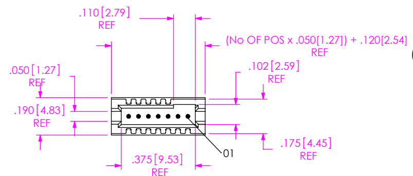
FIG 1 -S: SINGLE END (TFSSX-07-28-XX-XX.XX-S SHOWN)
