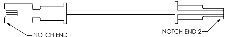
T-NDS (END 2 NOTCH DOWN, CABLE STRAIGHT) (PIN 1 TO PIN 1)
