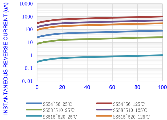
Fig.3-TYPICAL REVERSE CHARACTERISTICS
