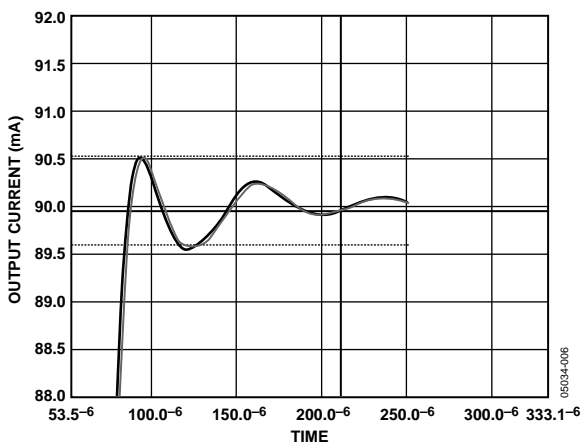
Figure 7. ¼ to ¾ Scale Settling Time (VDD = 3.6 V)
