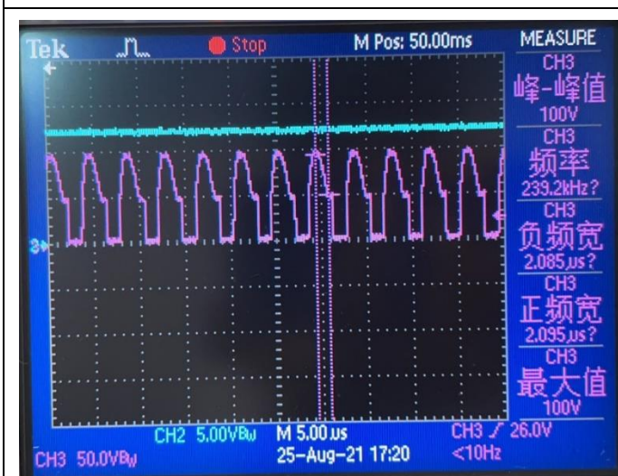
Switch Waveform
