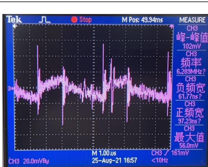
Full load ripple
