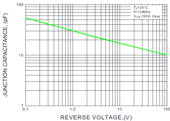
FIG.5-TYPICAL JUNCTION CAPACITANCE
