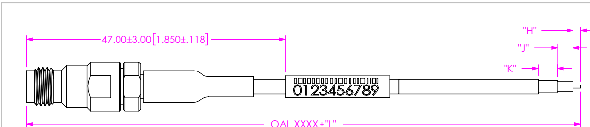
FIG 8 RF23C-24SJ-102030-XXXX SHOWN (SEE NOTE 8 & 9)
