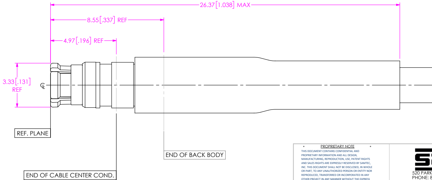
FIG 12 -00SJ SHOWN (PROTECTIVE CAP NOT SHOWN FOR CLARITY)
