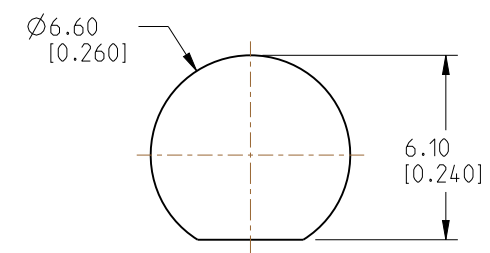
RECOMMENDED MOUNTING HOLE DIMNSIONS
