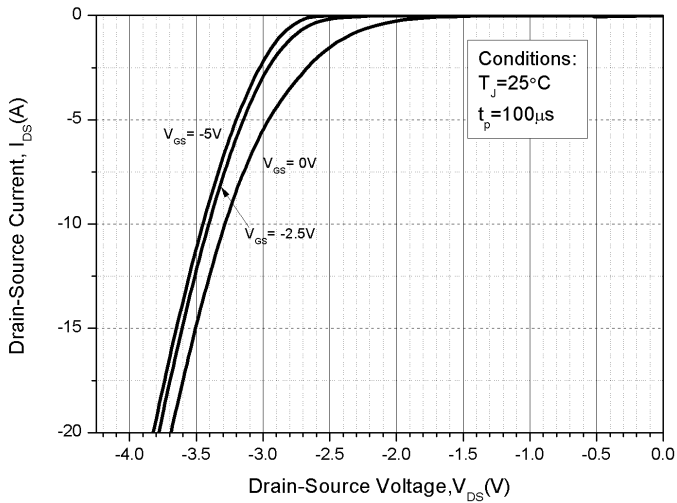
Figure 7. Body Diode Characteristics, T_J = 25\text{ }^\circ\text{C}
