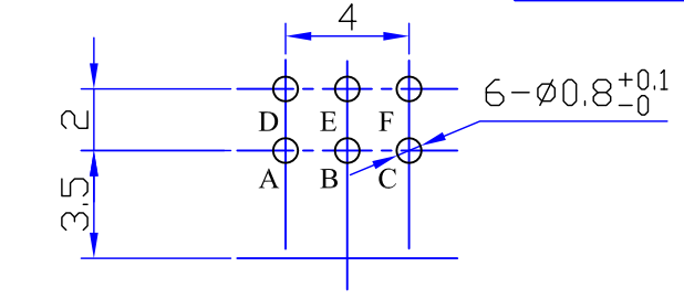
PCB Mounting Hole Detail
