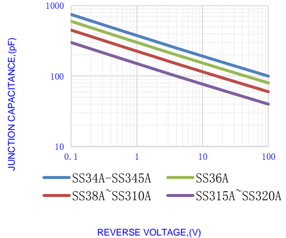
Fig.4-TYPICAL JUNCTION CAPACITANCE
