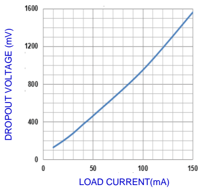
Fig.5-MAX. DROPOUT VOLTAGE VS. LOAD CURRENT
