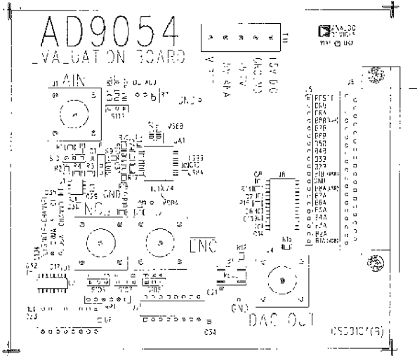
Figure 39. Assembly—Top View
