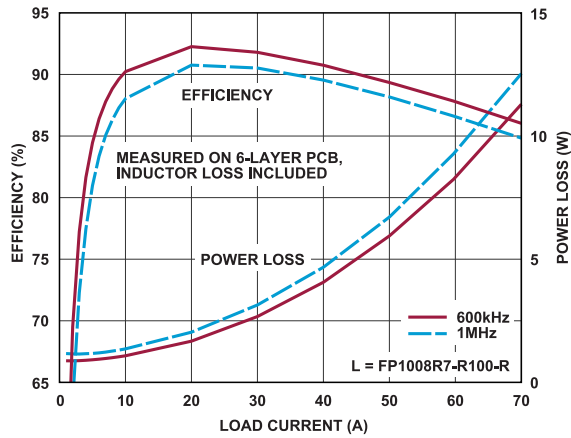
Figure 4. 12 V_{IN} to 1 V_{OUT} Efficiency
