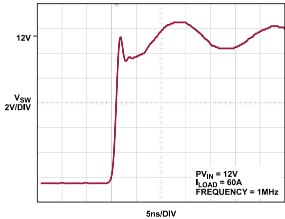
Figure 5. V_{SW} Waveform at 1 MHz
