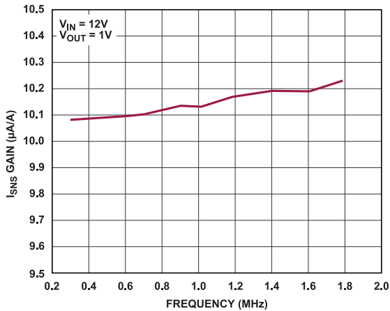
Figure 12. I_{SNS} Gain vs. Frequency
