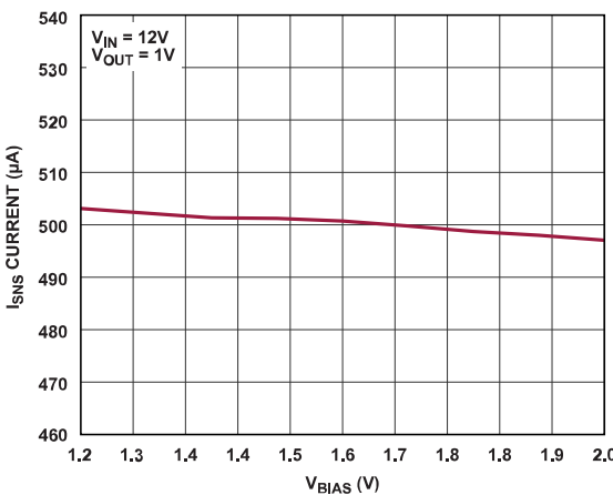
Figure 9. I_{SNS} Current vs. V_{BIAS}
