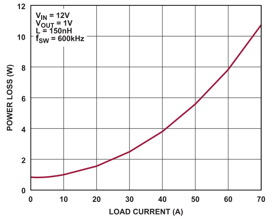
Figure 7. LTC7051-1 Power Dissipation vs. Load
