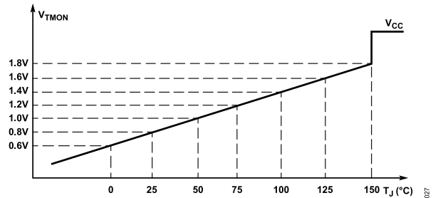
Figure 25. V_{TMON} vs. Die Temperature
