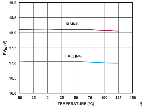
Figure 19. PV_{IN} OVLO vs. Temperature
