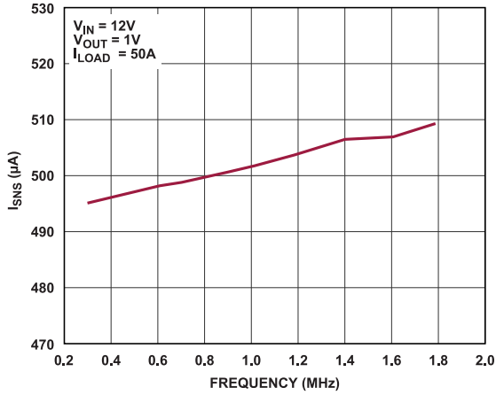
Figure 10. I_{SNS} vs. Frequency
