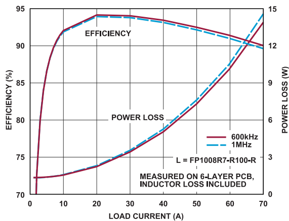
Figure 6. 12 V_{IN} to 1.8 V_{OUT} Efficiency
