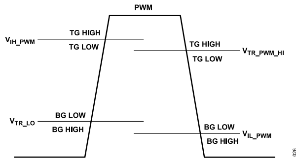
Figure 24. Three-State Input Operation
