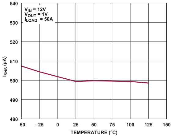
Figure 11. I_{SNS} vs. Temperature
