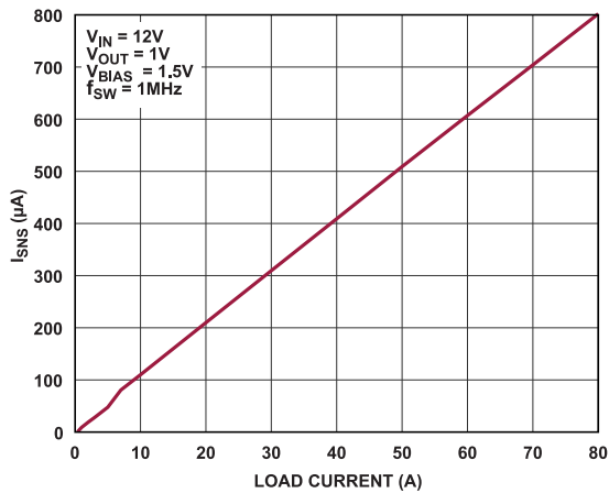
Figure 8. I_{SNS} vs. Load
