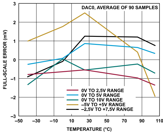
Figure 29. Full-Scale Error vs. Temperature
