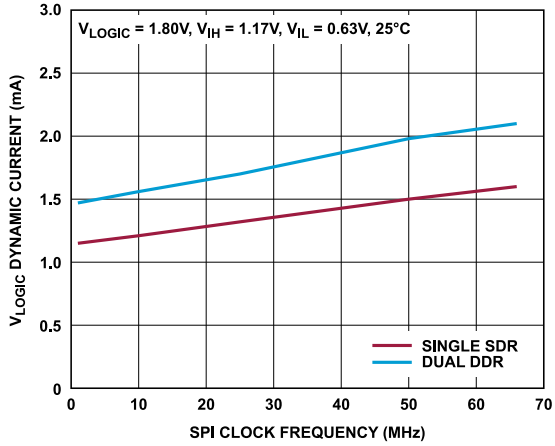
Figure 70. V_{Logic} Dynamic Current vs. SPI Clock Frequency, SPI Mode
