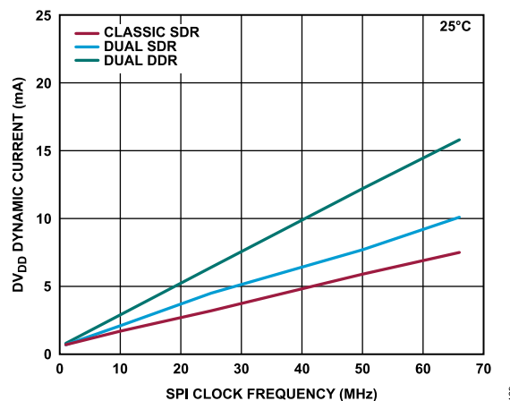
Figure 69. AD3541R-12 DV DD Dynamic Current vs. SPI Clock Frequency, SPI Mode
