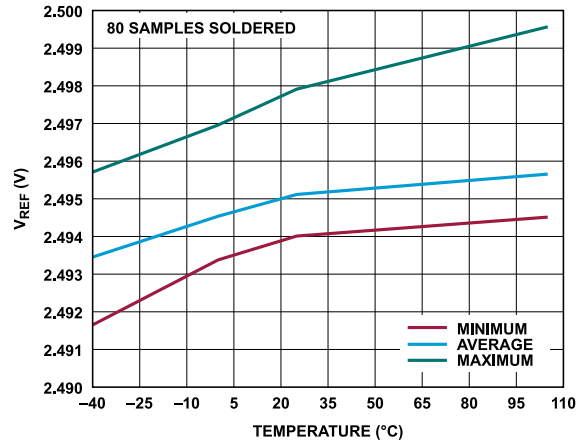
Figure 67. V REF vs. Temperature
