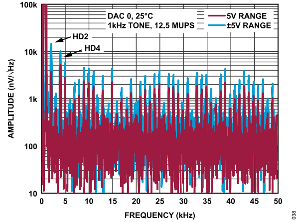
Figure 37. AD3541R-12 Spectral Noise Density with 1 kHz Sine Wave Playback
