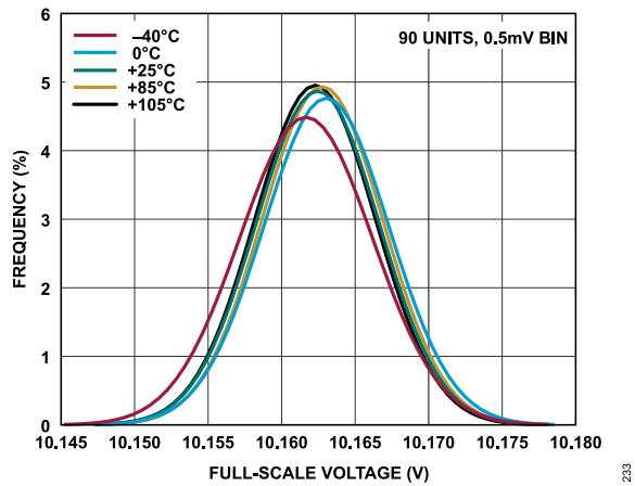
Figure 47. Full-Scale Voltage Distribution, 0 V to 10 V Range
