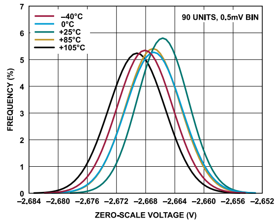
Figure 44. Zero-Scale Voltage Distribution, -2.5 V to +7.5 V Range
