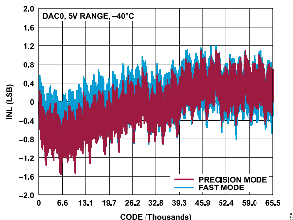
Figure 15. AD3541R-16 INL vs. Code, 0 V to 5 V Range, -40°C, Fast Mode and Precision Mode
