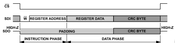
Figure 86. Basic SPI Write Frame with CRC
