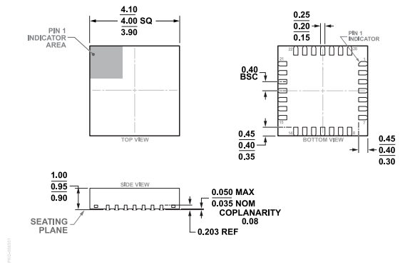
Figure 98. 28-Lead Lead Frame Chip Package [LFCSP] 4 mm x 4 mm Body and 0.95 mm Package Height (CP-28-15) Dimensions shown in millimeters
