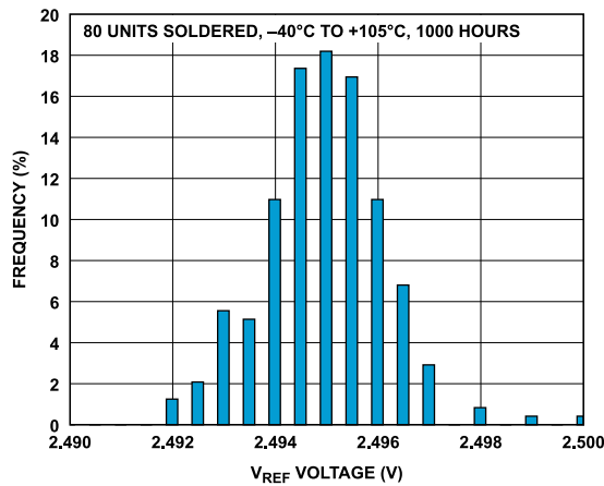
Figure 66. Reference Voltage Spread
