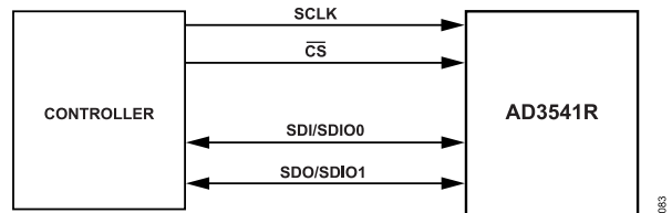
Figure 90. Dual SPI Connection
