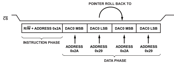
Figure 85. Looping Enabled with Address Descending and STREAM\_MODE = 2
