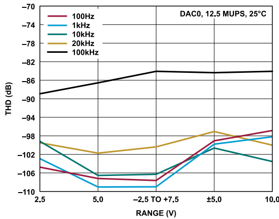
Figure 35. AD3541R-16 THD vs. Range
