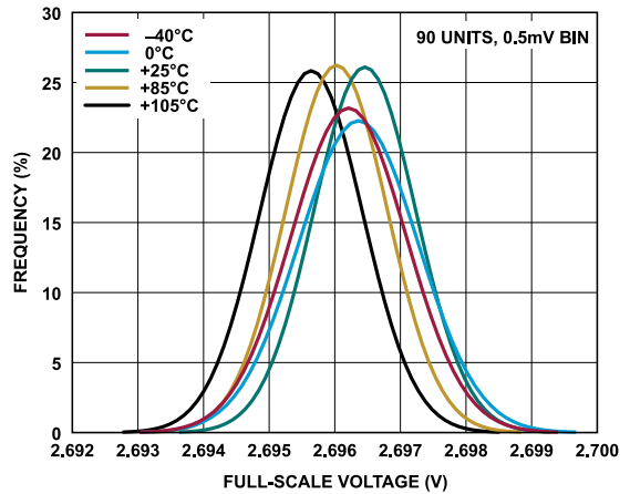
Figure 45. Full-Scale Voltage Distribution, 0 V to 2.5 V Range
