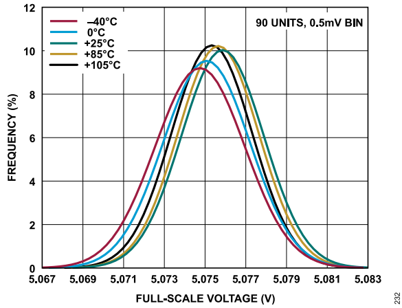
Figure 46. Full-Scale Voltage Distribution, 0 V to 5 V Range
