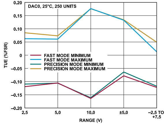
Figure 25. TUE vs. Range
