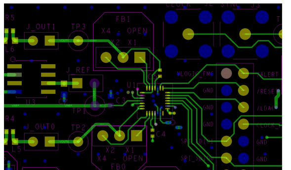
Figure 97. EVAL-AD3542R Component Arrangement and Layout
