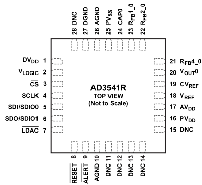
Figure 9. Pin Configuration
