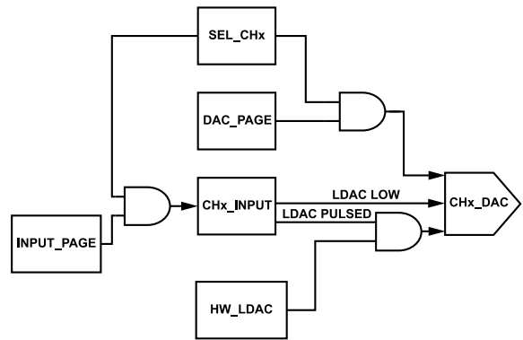
Figure 94. DAC Data Flow Between Registers
