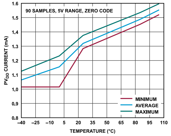
Figure 74. PV_{DD} Current vs. Temperature
