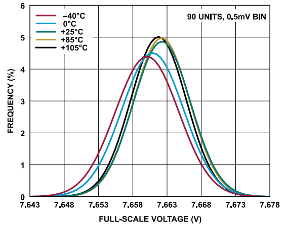
Figure 49. Full-Scale Voltage Distribution, -2.5 V to +7.5 V Range
