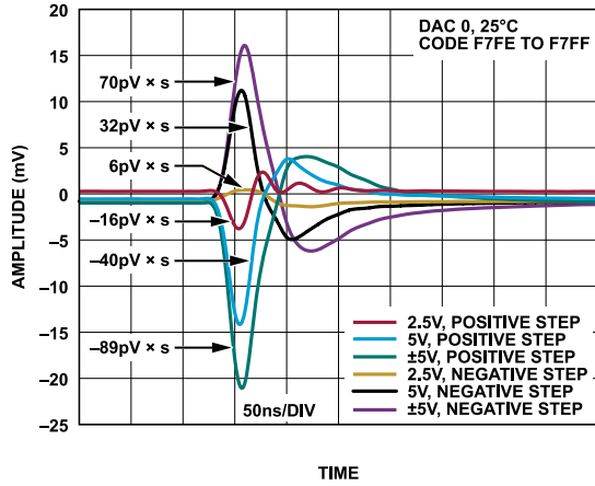
Figure 52. Digital-to-Analog Glitch
