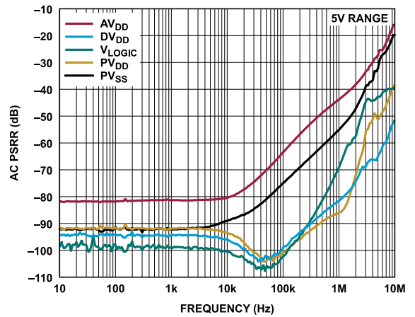
Figure 62. AC PSRR vs. Frequency
