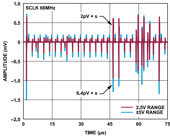
Figure 54. Digital Feedthrough
