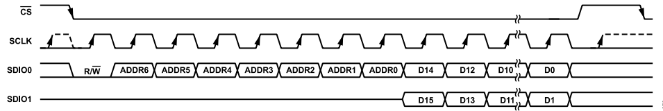
Figure 91. Dual SPI Mode
