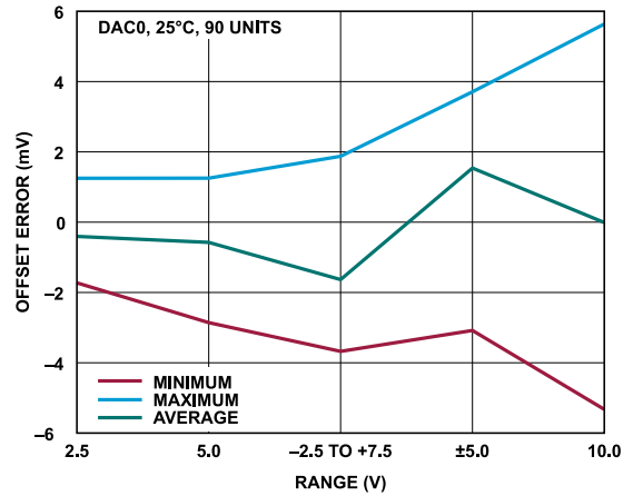
Figure 26. Offset Error vs. Range
