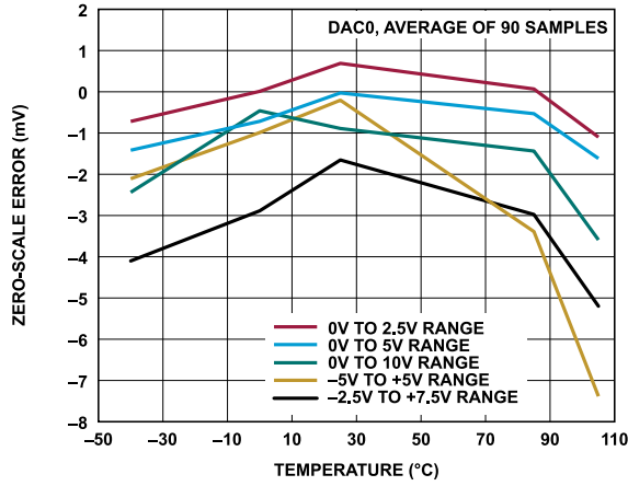
Figure 28. Zero-Scale Error vs. Temperature
