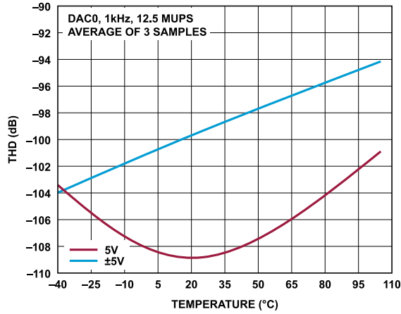
Figure 34. AD3541R-16 THD vs. Temperature
