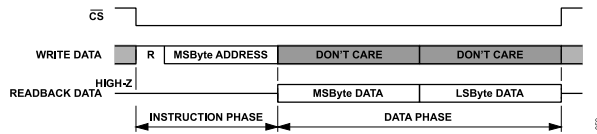
Figure 81. Multibyte Register Read with Descending Addressing
