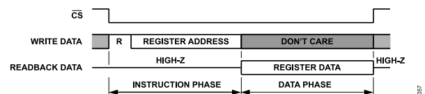
Figure 79. Basic SPI Read Frame
