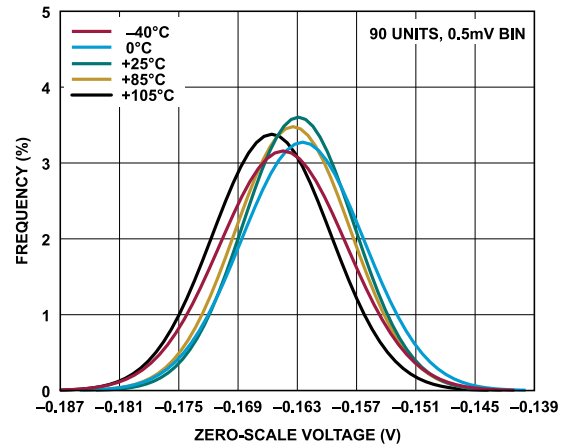
Figure 42. Zero-Scale Voltage Distribution, 0 V to 10 V Range
