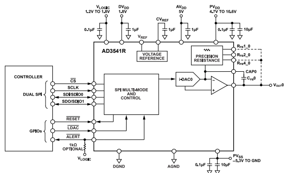
Figure 96. Recommended Application Circuit
