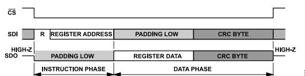
Figure 87. Basic SPI Read Frame with CRC
