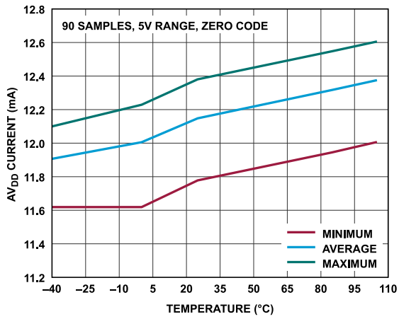
Figure 71. AV_{DD} Current vs. Temperature
