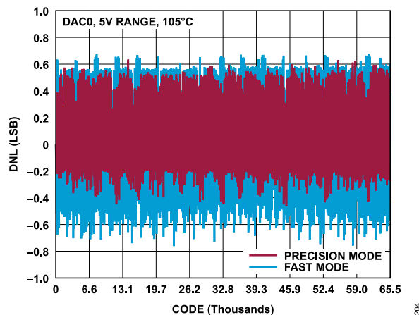
Figure 13. AD3541R-16 DNL vs. Code, 0 V to 5 V Range, 105°C, Fast Mode and Precision Mode
