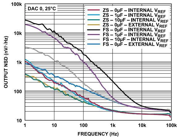
Figure 30. Output Noise Spectral Density (NSD) vs. Frequency
