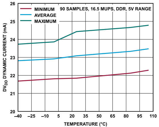
Figure 72. AD3541R-16 DV_{DD} Dynamic Current vs. Temperature
