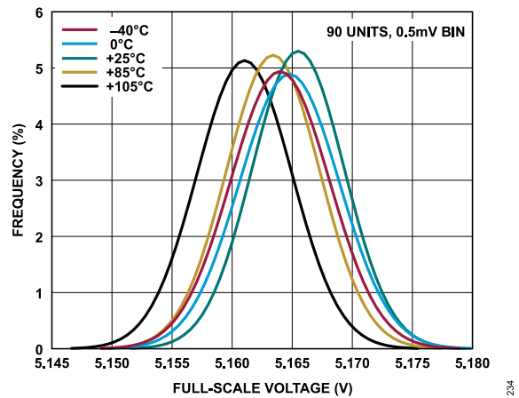
Figure 48. Full-Scale Voltage Distribution, -5 V to +5 V Range
