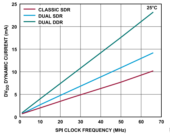
Figure 68. AD3541R-16 DV DD Dynamic Current vs. SPI Clock Frequency, SPI Mode
