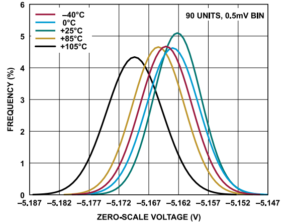
Figure 43. Zero-Scale Voltage Distribution, -5 V to +5 V Range
