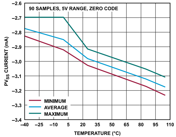
Figure 75. PV_{SS} Current vs. Temperature
