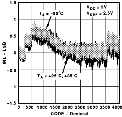
Figure 4. AD7394 Integral Nonlinear Error vs. Code
