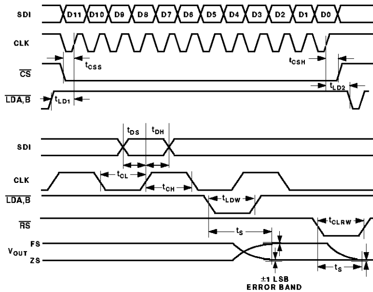
Figure 2. Timing Diagram
