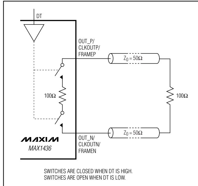
Figure 8. Double-Termination
