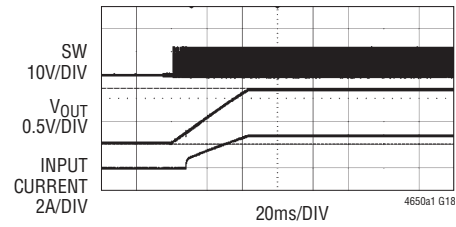
Single Phase Start-up with 25A Load
