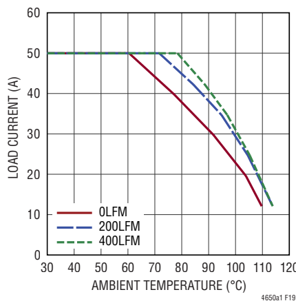
Figure 19. 12V to 1V Derating Curve, No Heat Sink
