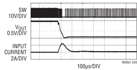
Single Phase Short Circuit Protection with 25A Load
