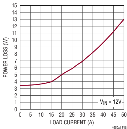
Figure 18. 5V OUT Power Loss Curve
