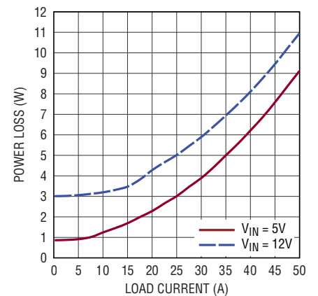
Figure 17. 3.3V OUT Power Loss Curve
