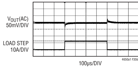
25% Load Step Transient Response ±3% Output Regulation Window. 12VIN, 1.0VOUT, 50A per Above Circuit
