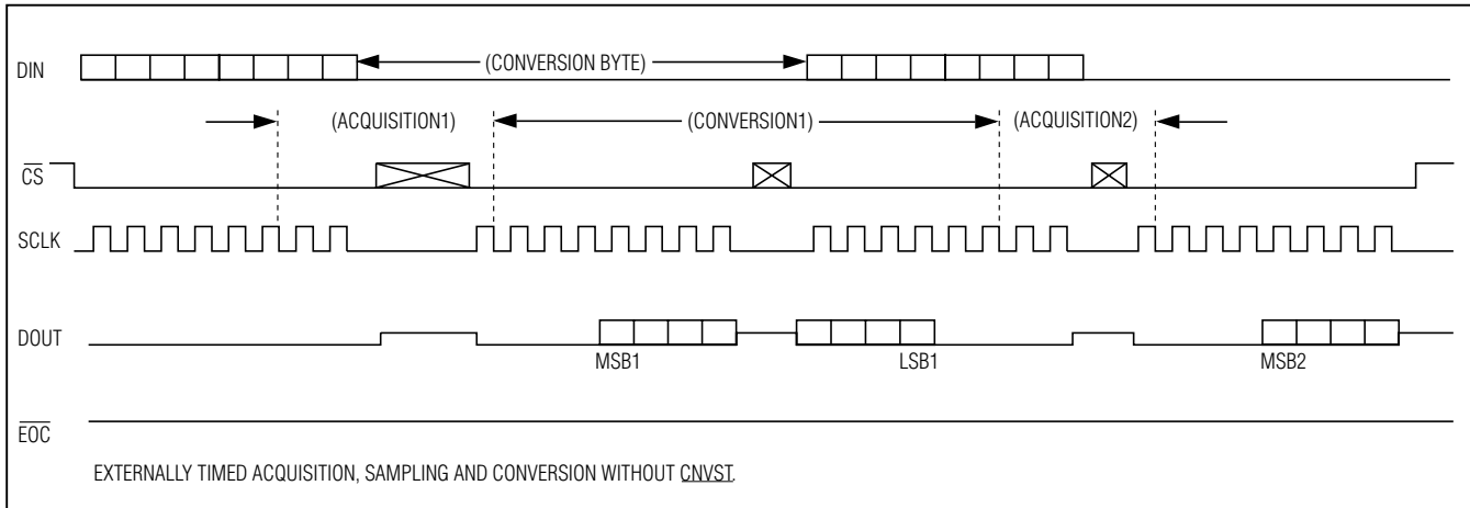
Figure 7. Clock Mode 11
