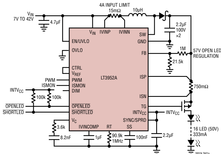
Short-Circuit Robust Boost LED Driver with Spread Spectrum Frequency Modulation
