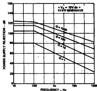
Figure 13. Positive PSRR vs. Frequency
