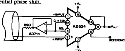
Figure 35. Shield Driver, G ≥ 100
