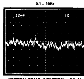
Figure 18. Low Frequency Noise - G = 1000 (System Gain = 100,000)
