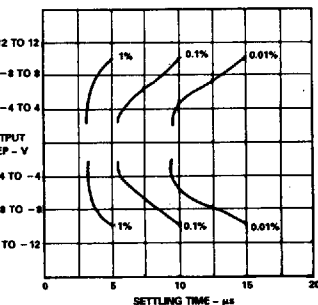
Figure 19. Settling Time Gain = 1
