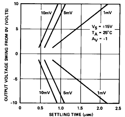
SETTLING TIME
