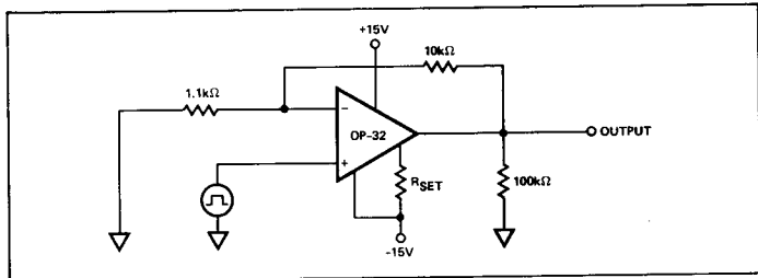
TEST CIRCUIT
