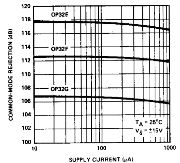
COMMON-MODE REJECTION vs SUPPLY CURRENT
