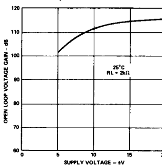
Figure 11. Open Loop Voltage Gain vs. Supply Voltage
