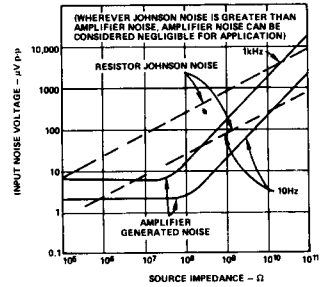
Figure 18. Total RMS Noise vs. Source Impedance
