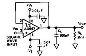
Figure 21c. Unity Gain Follower
