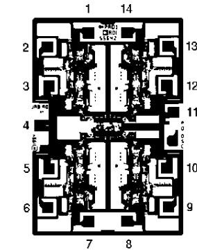
OP496 Die Size 0.062 × 0.092 inch, 5,704 sq. mils Substrate (Die Backside) Is Connected to V+. Transistor Count, 214.
