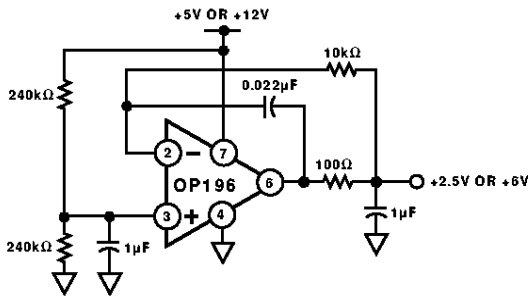
Figure 41. A Micropower False-Ground Generator
