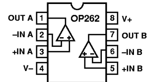
8-Lead Plastic DIP (P Suffix)
