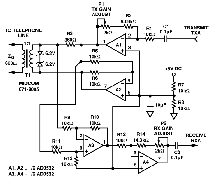
Figure 44. A Single-Supply Direct Access Arrangement for Modems
