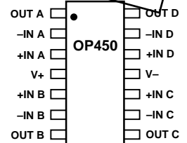
14-Lead SO ($ Suffix)
