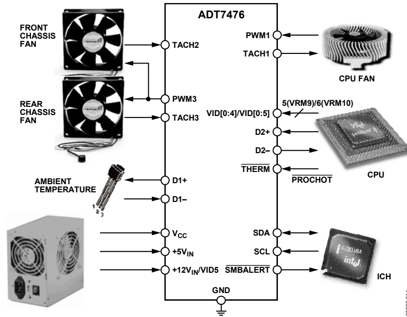
Figure 13. ADT7476 Configuration
