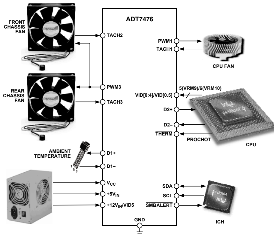
Figure 49. Recommended Implementation 1
