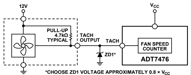
Figure 42. Fan with TACH Pull-Up to Voltage > 3.6 V (for Example, 12 V), Clamped with Zener Diode
