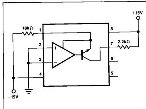
BURN-IN CIRCUIT
