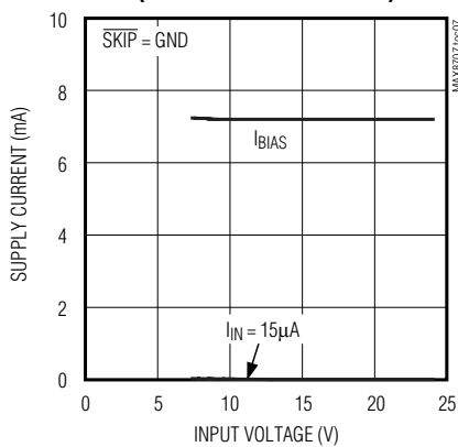
NO-LOAD SUPPLY CURRENT vs. INPUT VOLTAGE (1-PHASE PULSE SKIPPING)
