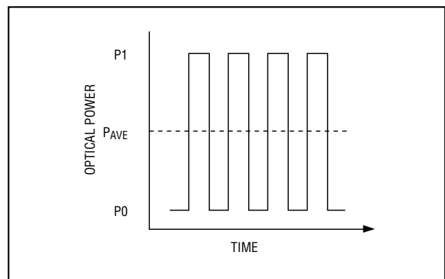
Figure 2. Optical-Power Definitions
