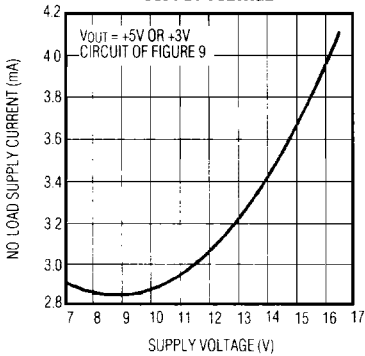
MAX741D STEP-DOWN NO-LOAD SUPPLY CURRENT vs. SUPPLY VOLTAGE
