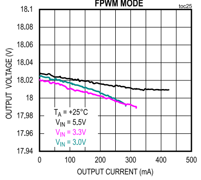
LOAD REGULATION vs. INPUT VOLTAGE 18V OUT FPWM MODE
