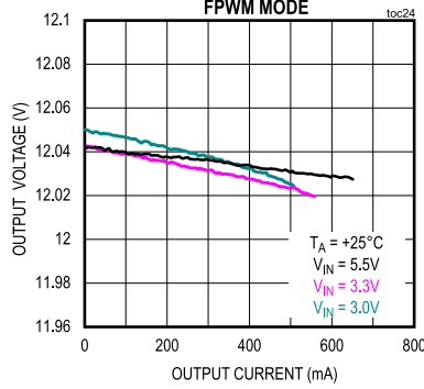
LOAD REGULATION vs. INPUT VOLTAGE 12V OUT FPWM MODE
