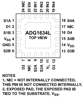
Figure 2. Pin Configuration
