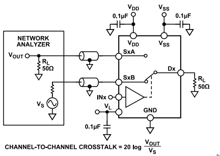
Figure 31. Channel-to-Channel Crosstalk
