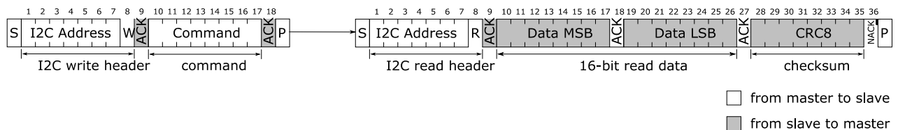
Figure 11: I2C transfer types: First a write header is sent to the I2C slave, followed by a command, for example “measure RH&T with highest precision”. After the measurement is finished the read request directed to this I2C slave will be acknowledged and transmission of data will be started by the slave.
