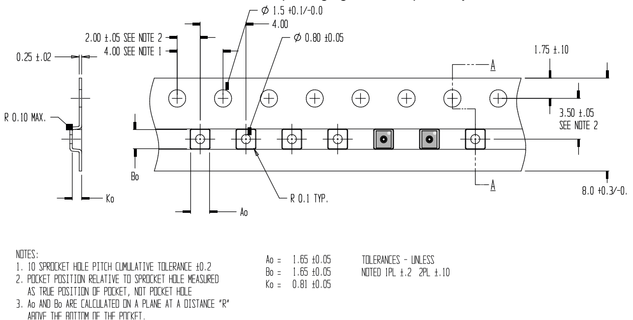
Figure 15: Tape and reel specifications including sensor orientation in pocket (see indication of two sensors on the right side of the tape).
