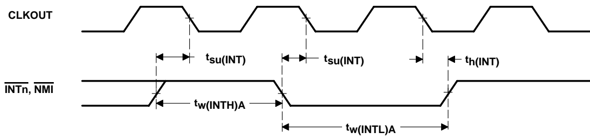
Figure 5–16. Interrupt Timing
