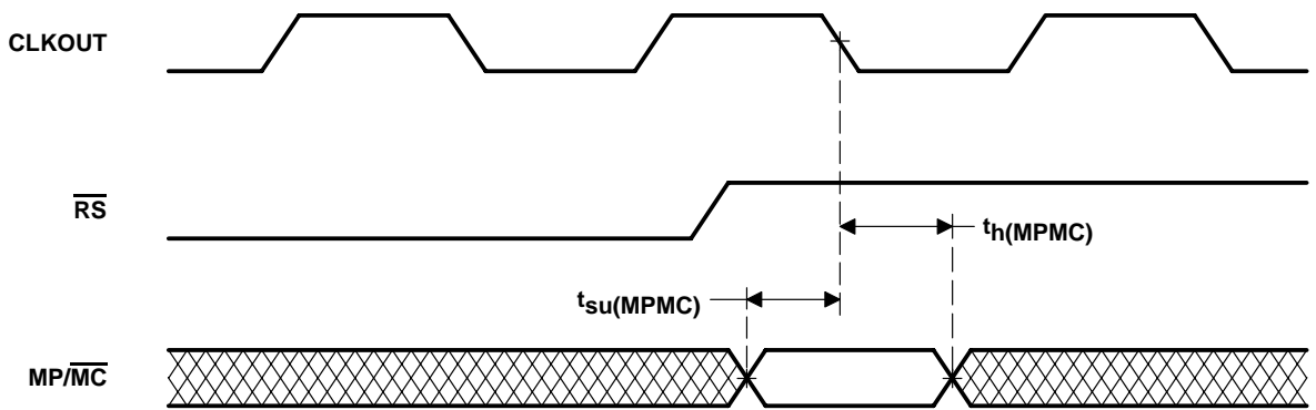
Figure 5–17. \overline{\text{MP/MC}} Timing
