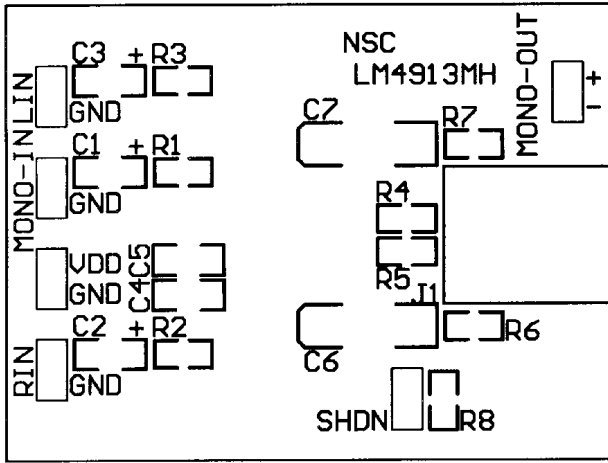
FIGURE 5. Top Overlay
