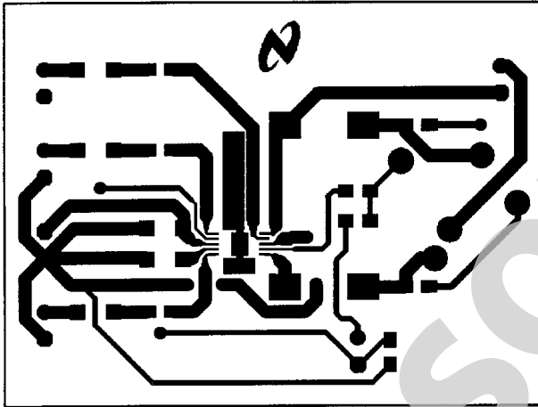
FIGURE 5. Top Overlay
