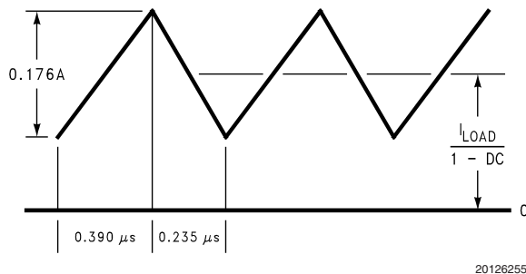
FIGURE 2. 10 \mu H Inductor Current 5V - 12V Boost (LM4805)
