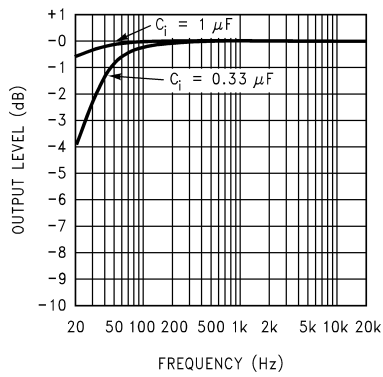
Amplifier Frequency Response vs Input Capacitor Size
