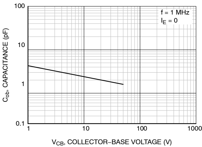
Figure 5. Output Capacitance
