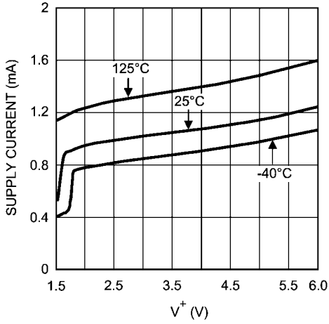
Supply Current vs. Supply Voltage (LMV793)
