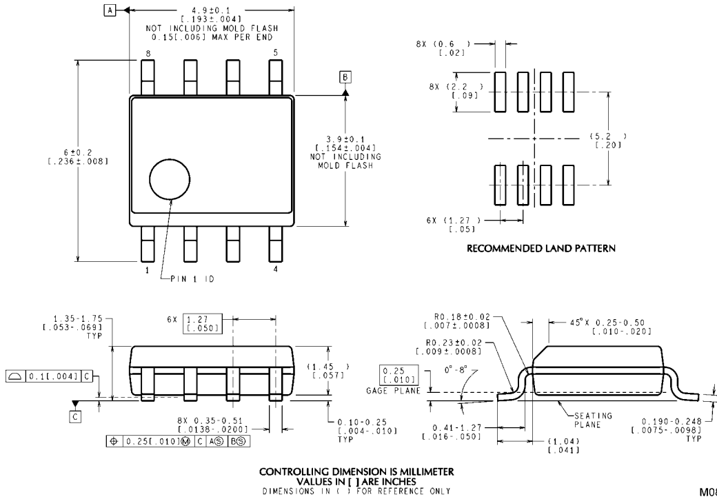
8-Pin SOIC NS Package Number M08A
