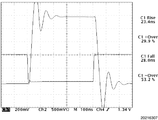
FIGURE 7. C Increased to 2.2 nF, Gain = -1
