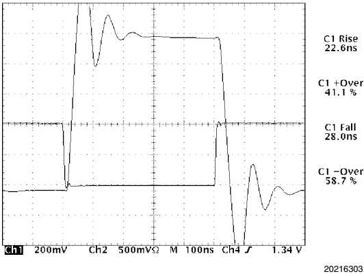
FIGURE 6. First Try at Compensation, Gain = -1
