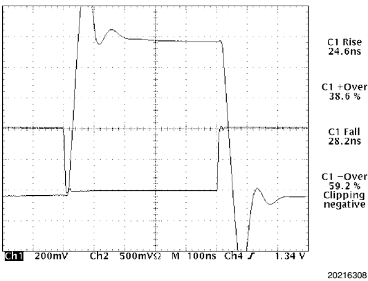
FIGURE 8. R_C = 240\Omega and C = 390 pF, Gain = -1
