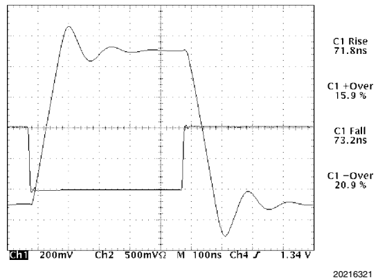
FIGURE 10. LMV796 Response
