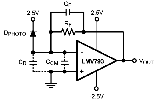
FIGURE 16. Transimpedance Amplifier
