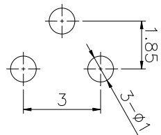
PCB. 焊接图 PCB. WELDING DRAWING
