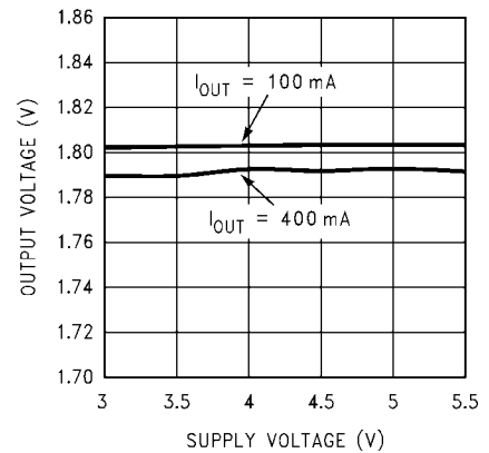
Output Voltage vs Supply Voltage ( V_{OUT} = 1.8V , PWM Mode)
