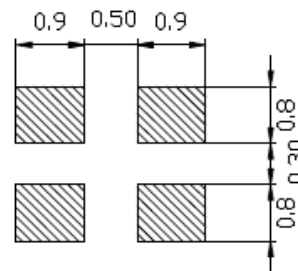
LAND PATTERN(REFERENCE)
