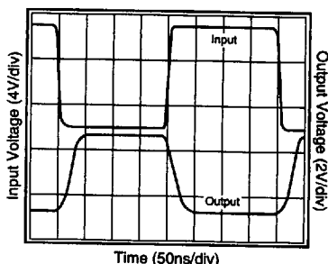
Figure 5: Overdrive Recovery
