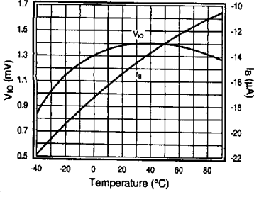
Is, Vo, vs. Temperature
