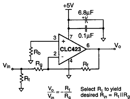
Figure 2: Inverting Configuration
