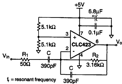
Figure 9: Bandpass Filter Topology
