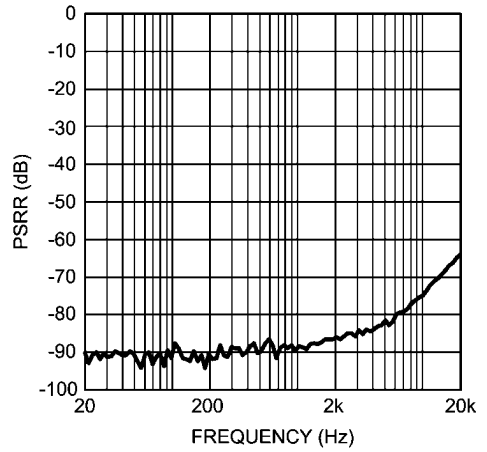
PSRR vs Frequency R_L = 32\Omega , V_{RIPPLE} = 200mV_{PP} on V_{DDLS} V_{DDLS} = 3.6V , C_B = 4.7\mu F , Mode 2, 10, HP
