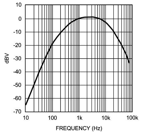
FIGURE 3. A-Weighted Filter
