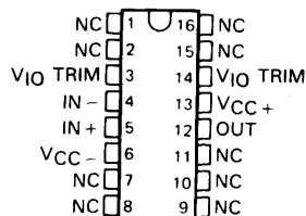
DW SMALL-OUTLINE PACKAGE (TOP VIEW)
