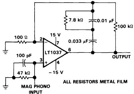
FIGURE 47. PHONO PREAMPLIFIER
