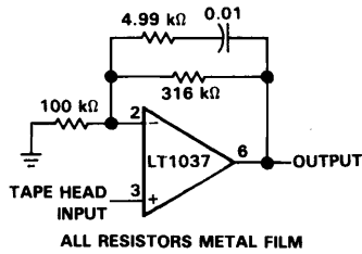
FIGURE 48. TAPE HEAD AMPLIFIER ALL RESISTORS METAL FILM
