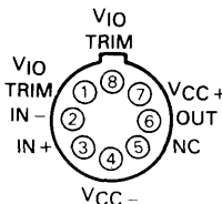
L PLUG-IN PACKAGE (TOP VIEW)
