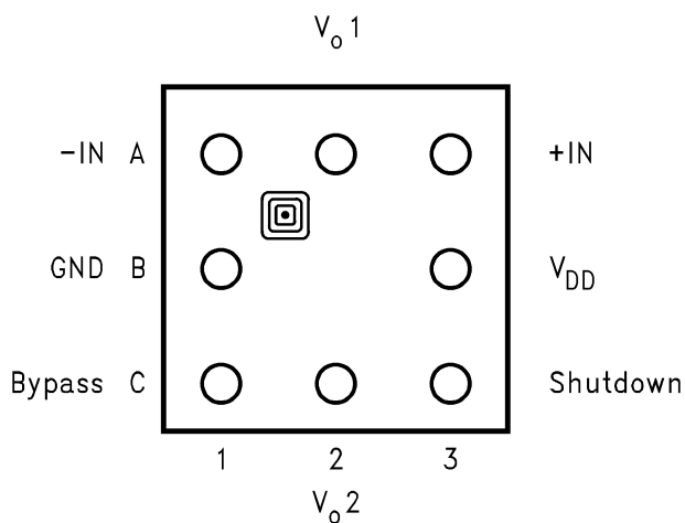
8 Bump DSBGA (Top View) See Package Number YZR
