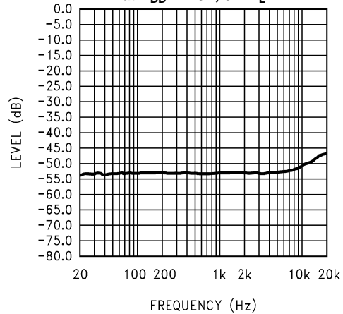
Figure 15. Input Floating
