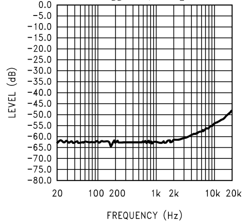
Figure 11. Input Floating
