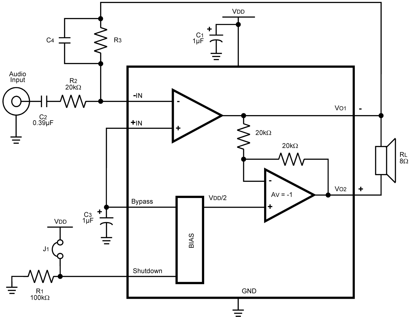
Figure 31. HIGHER GAIN AUDIO AMPLIFIER
