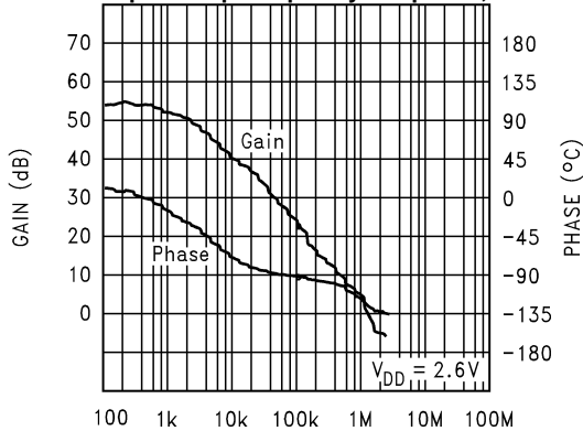
Open Loop Frequency Response, 2.6V
