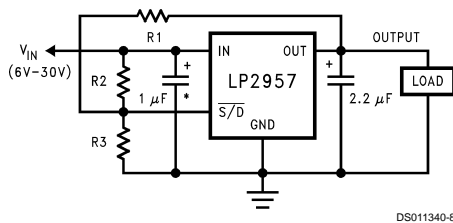
FIGURE 3. Snap-On/Snap-Off Output
