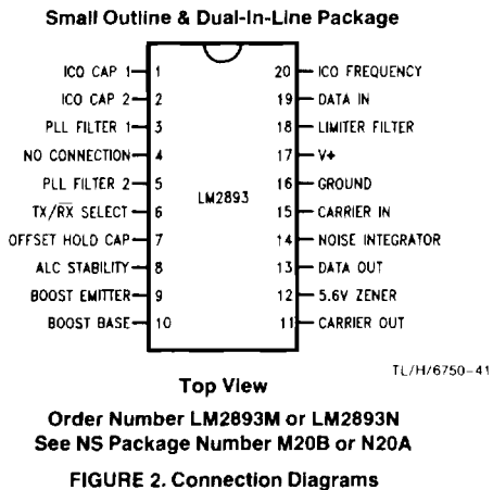
FIGURE 2. Connection Diagrams
