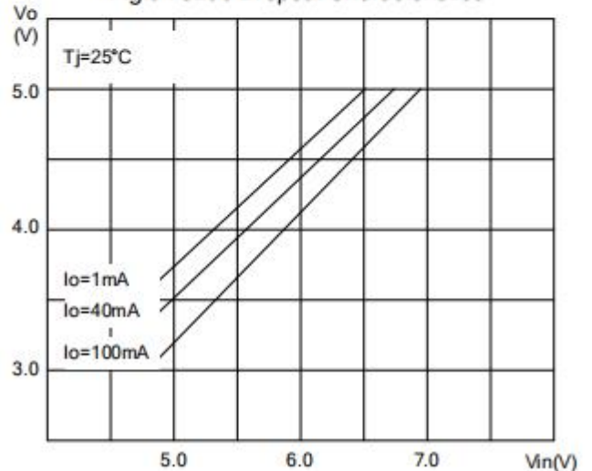
Fig.6 78L05 Dropout Characteristics
