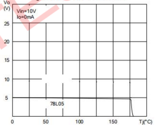
Fig.4 78L05 Thermal Shutdown
